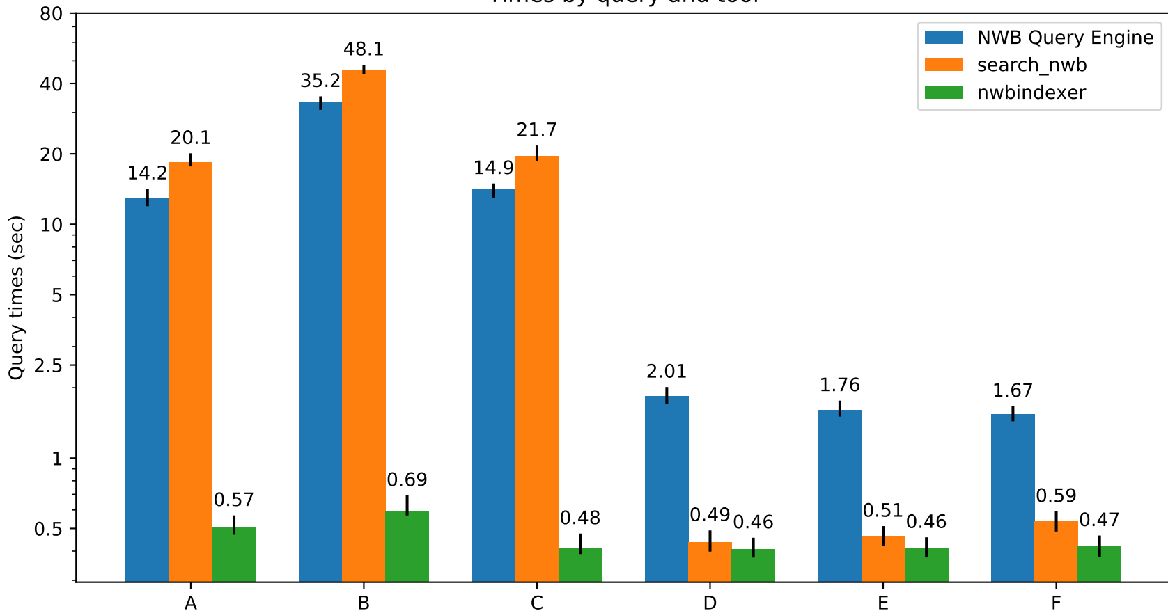
Times by query and tool
